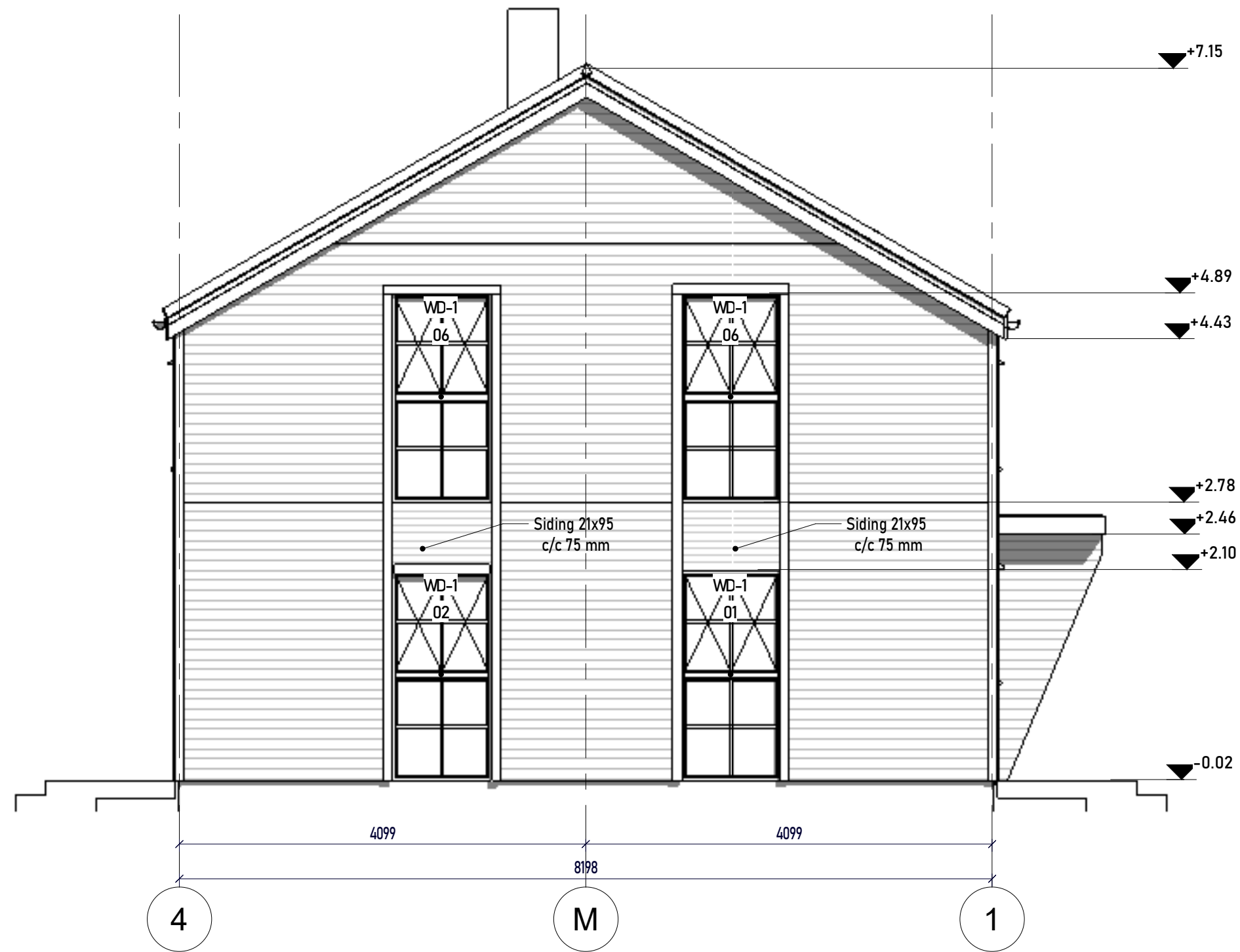
1 Facade 4-1 - South 1:50
